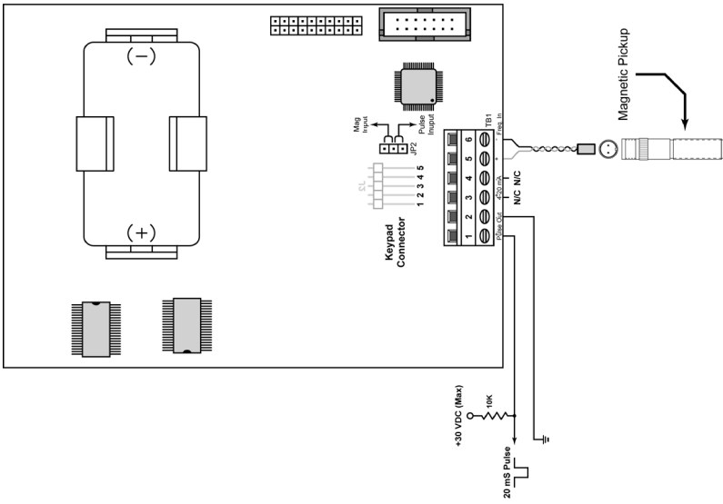
FIGURE 2 - CIRCUIT BOARD LAYOUT
